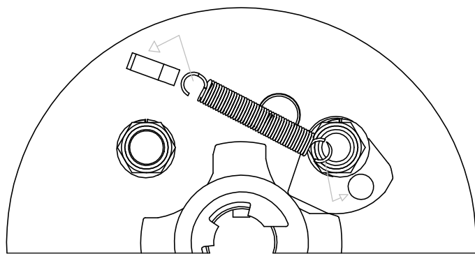
SPRING DETAIL
